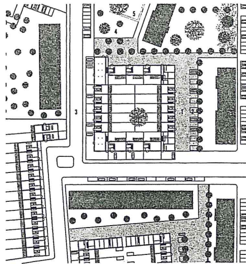
detail plan
