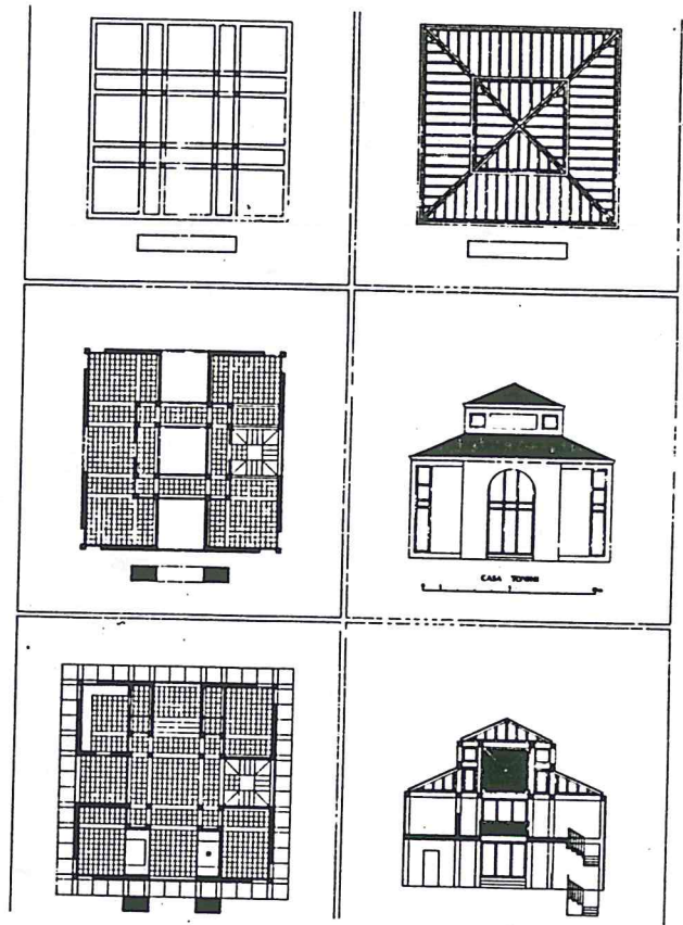
Casa Tonini View of the entrance elevation Plans and elevations
